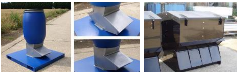
Figure 10. Examples of covered feeders for outdoor use
